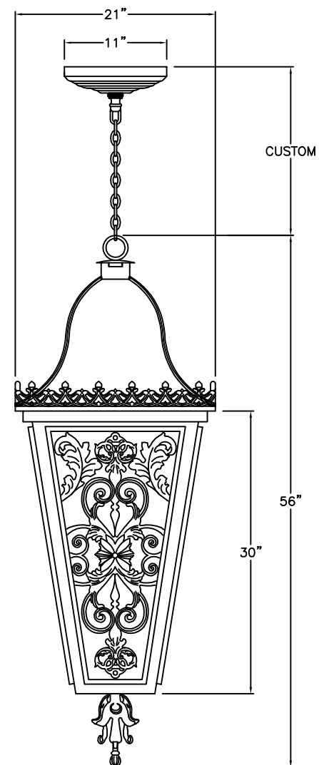
XLARGE E-002C-044 21" W X 56" H
