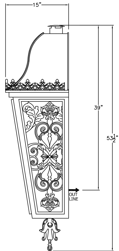
XLARGE E-002C-004 21" W X 53 1/2" H X 15" D
