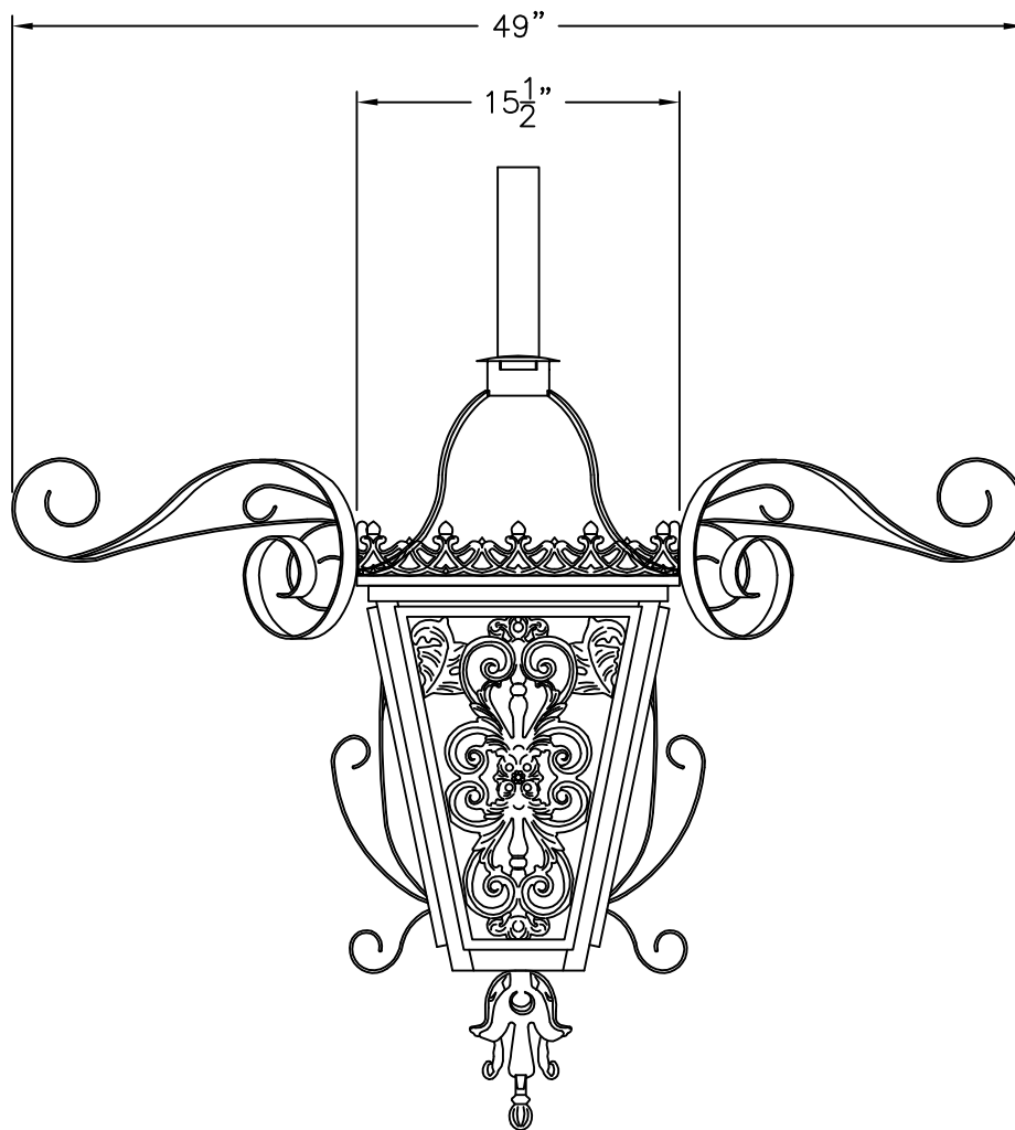
FRONT VIEW
