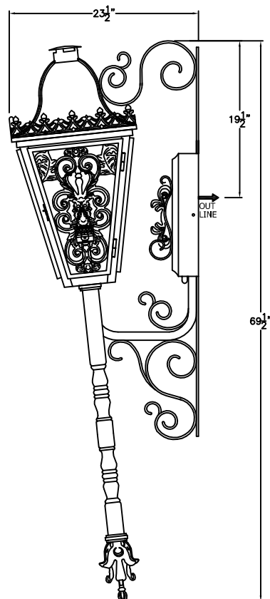
MEDIUM E-002C-082 15 1/2" W X 69 1/2" H X 23 1/2" D
