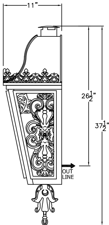
MEDIUM E-002C-002 15 1/2" W X 37 1/2" H X 11" D
